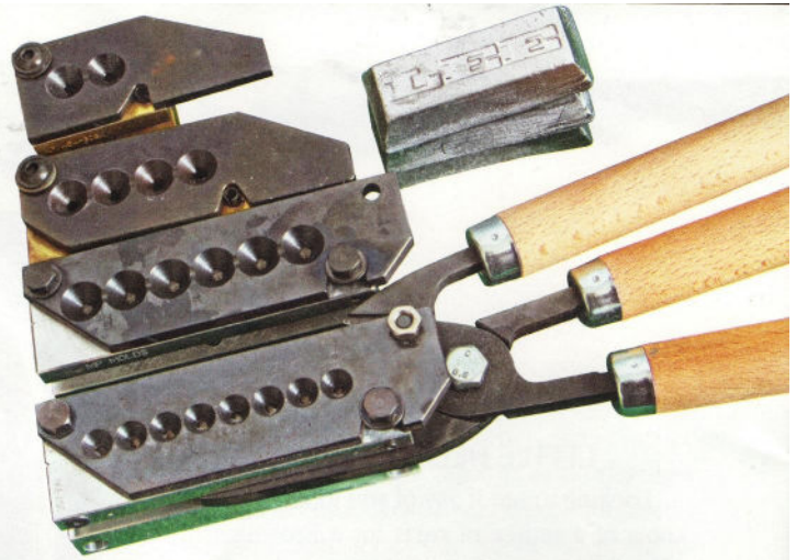
MP-Molds can be had in 2-, 4-, 6- and 8-cavity style. The more the merrier when it comes to casting.
